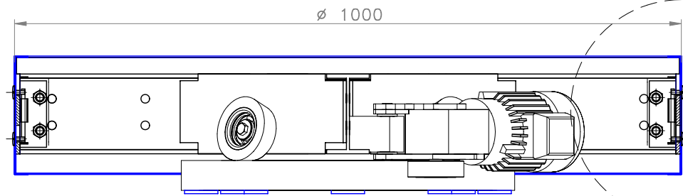
Detail A
